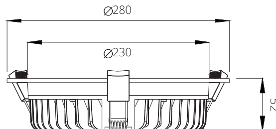
10" Downlight
