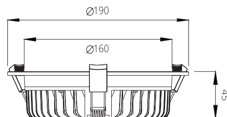
6" Downlight
