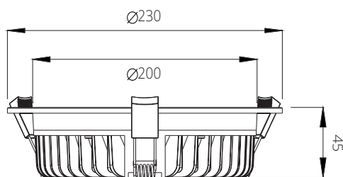
8" Downlight
