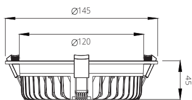
4" Downlight
