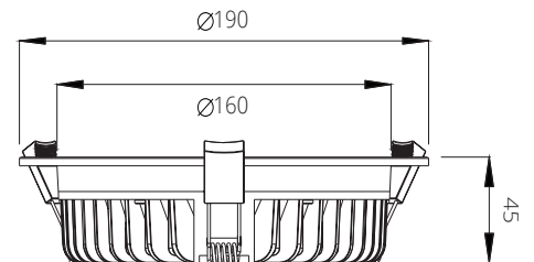
6" Downlight
