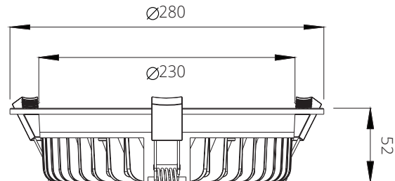
10" Downlight
